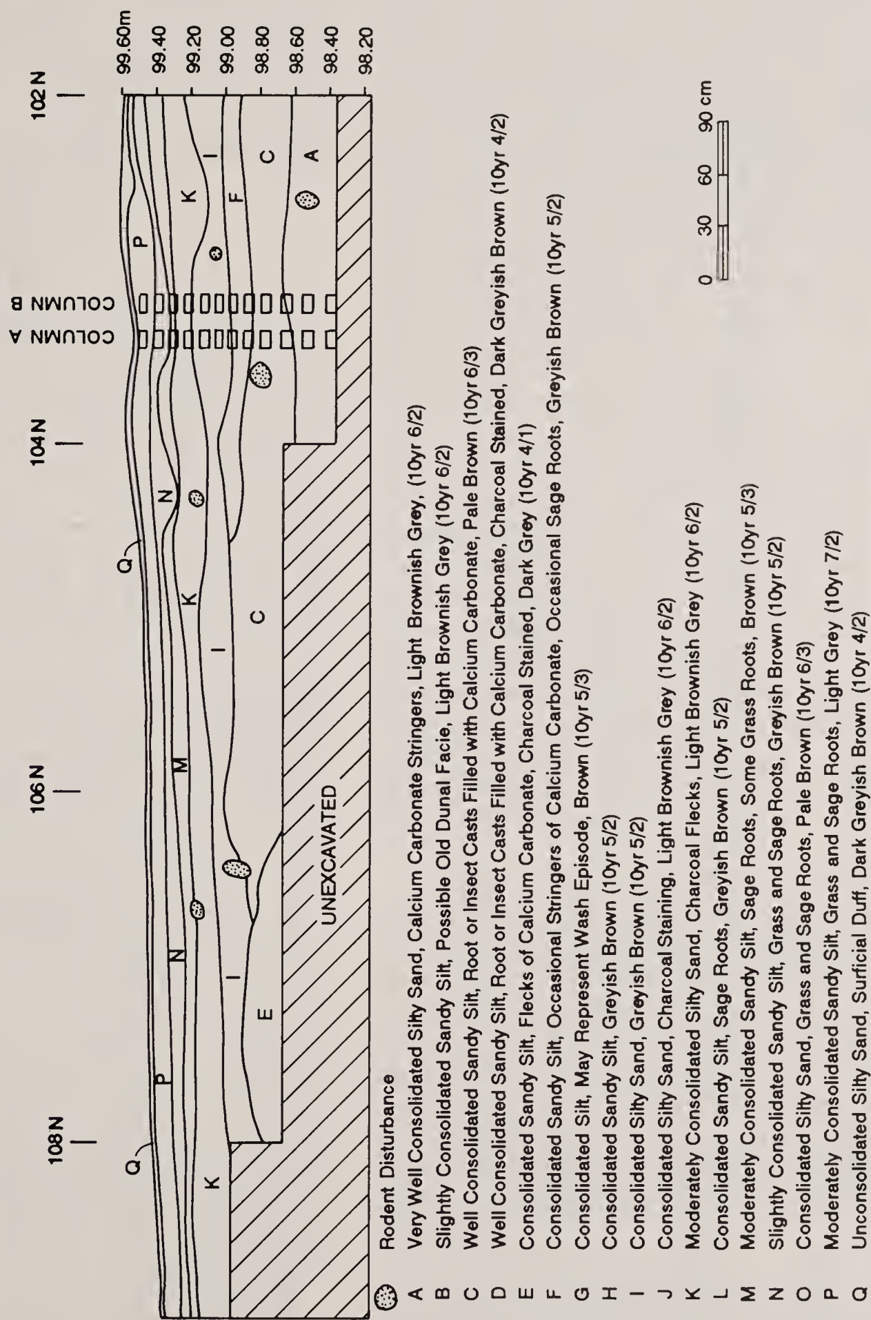
Figure 4.5 Profile of South wall of Excavation Block, Site 48CR4681 (Locality P-054).
