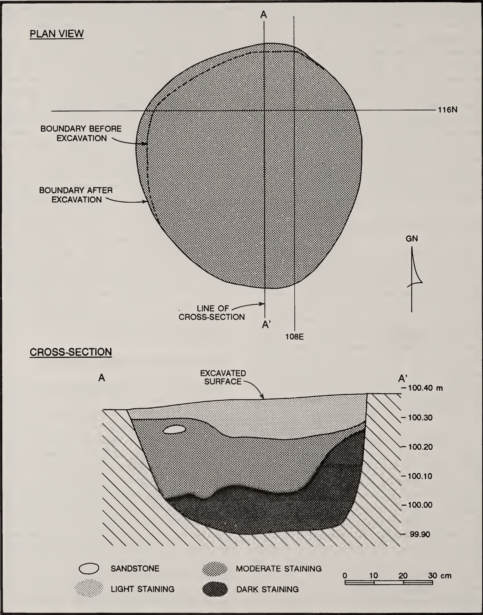
Figure 9.34 Plan View and Cross Section of Feature 33, Component II, Bald Knob Site.
