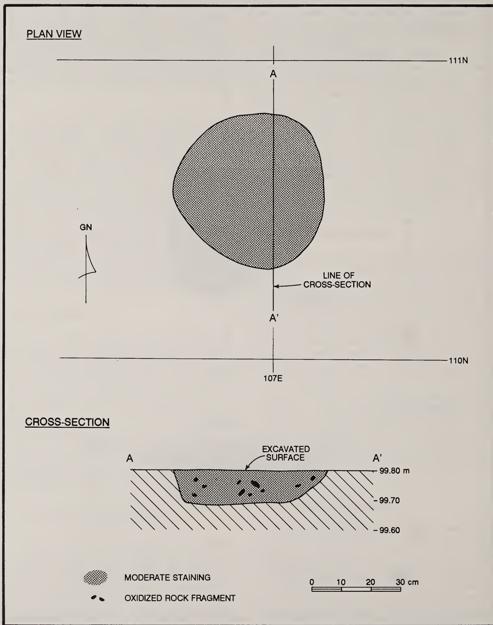
Figure 9.40 Plan View and Cross Section of Feature 21, Component II, Bald Knob Site.
