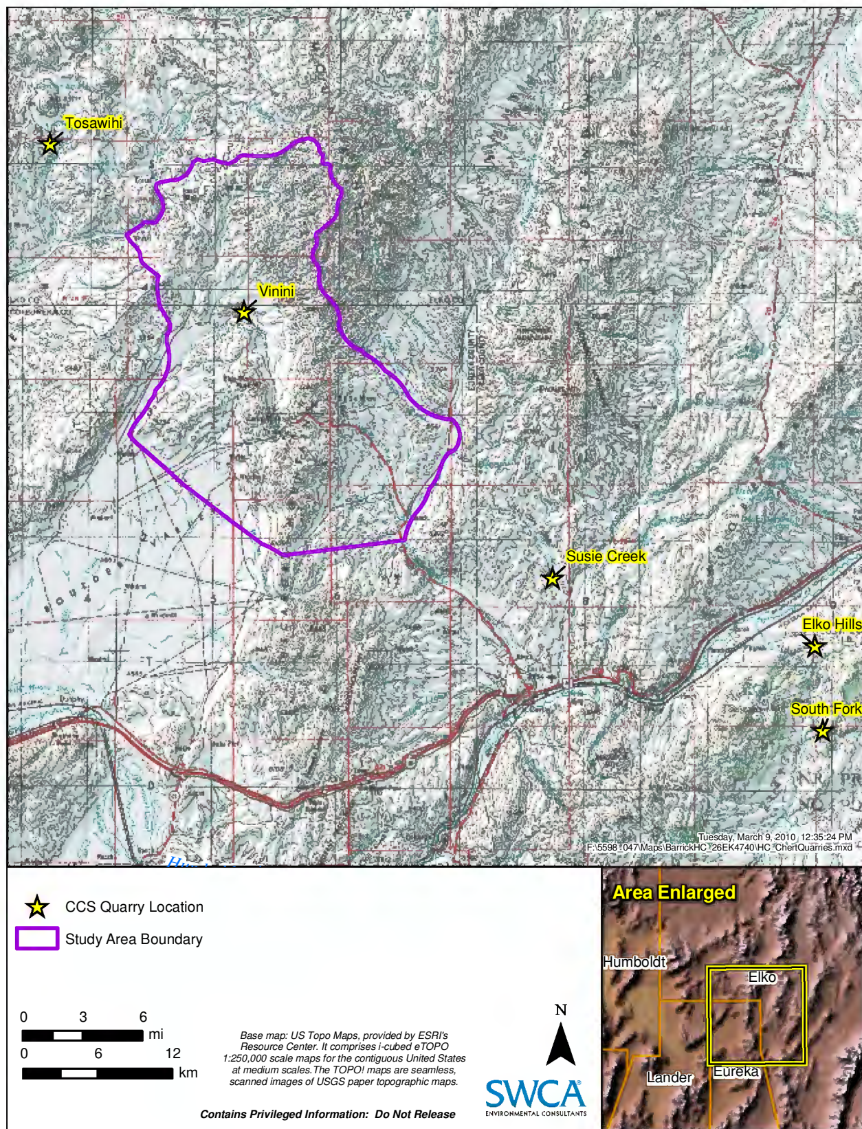
Figure 34. Location of the Tosawih Quarries and other sources of cryptocrystalline silicate (CCS) materials in relation to the LBB study area.
