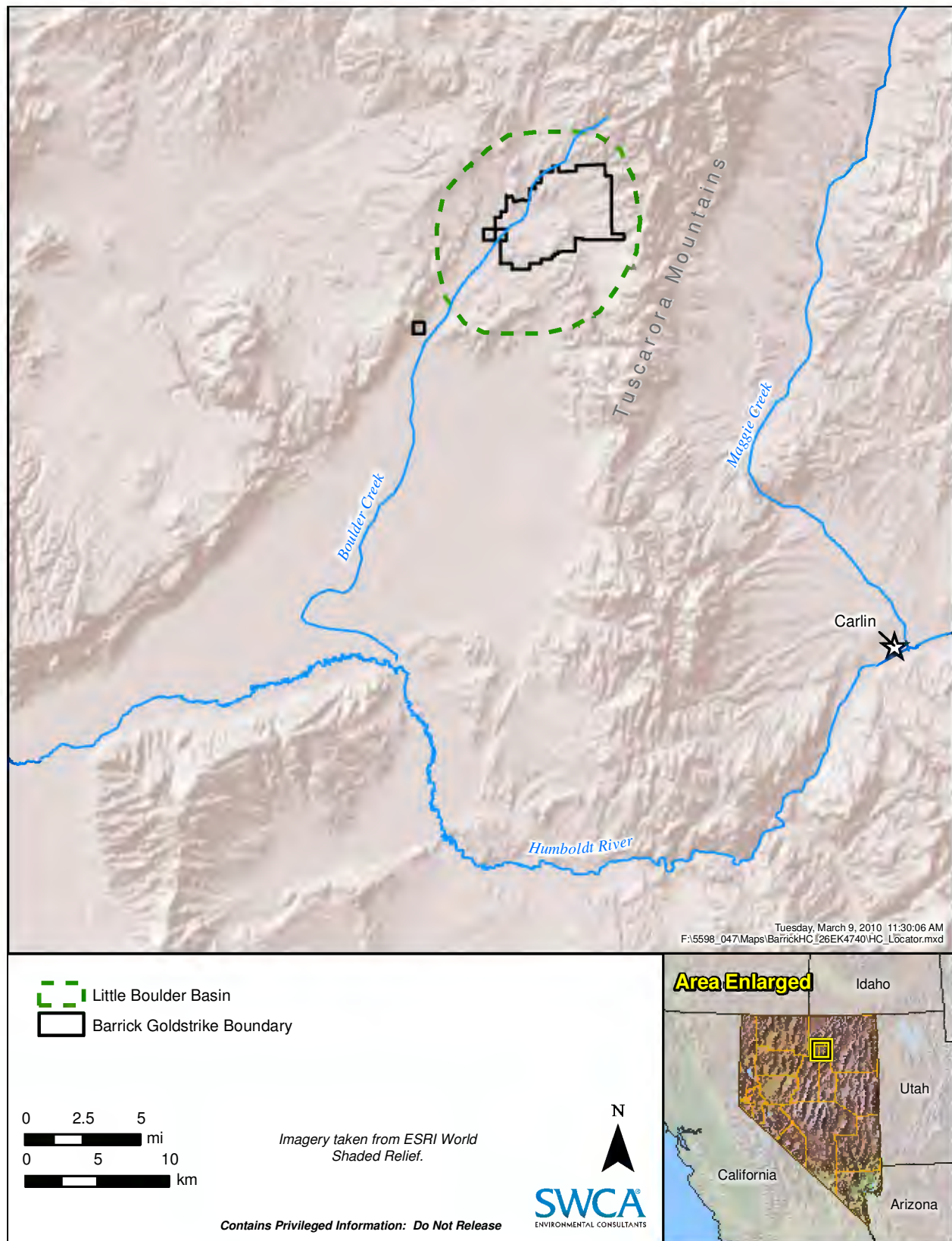
Figure 1. Location of the Little Boulder Basin and Barrick Goldstrike Mines in north-central Nevada.
