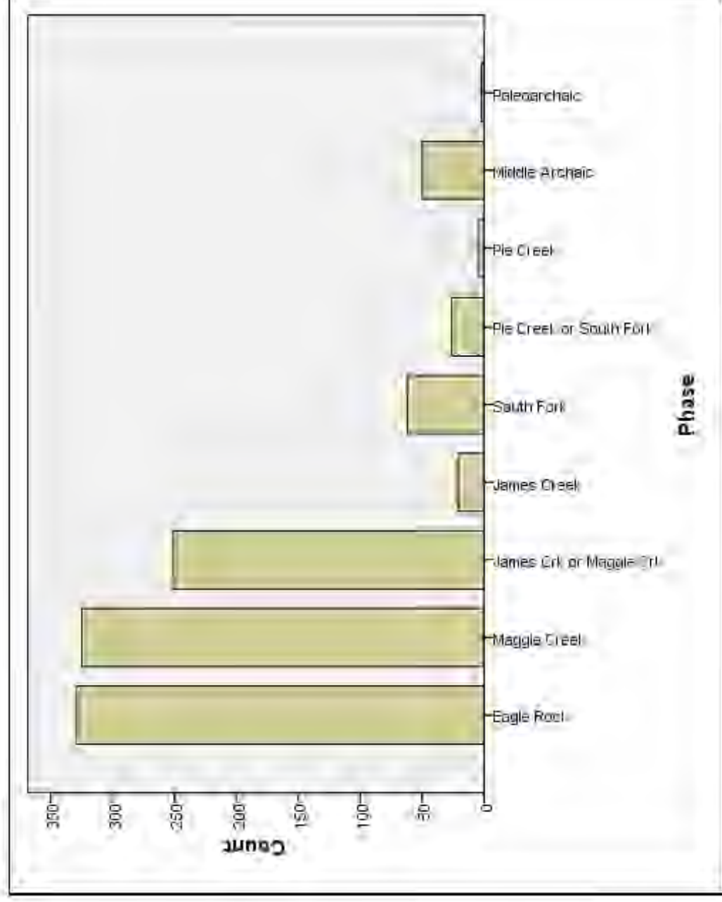
Figure 11. Distribution of all dating data from Table 19 by phase.
