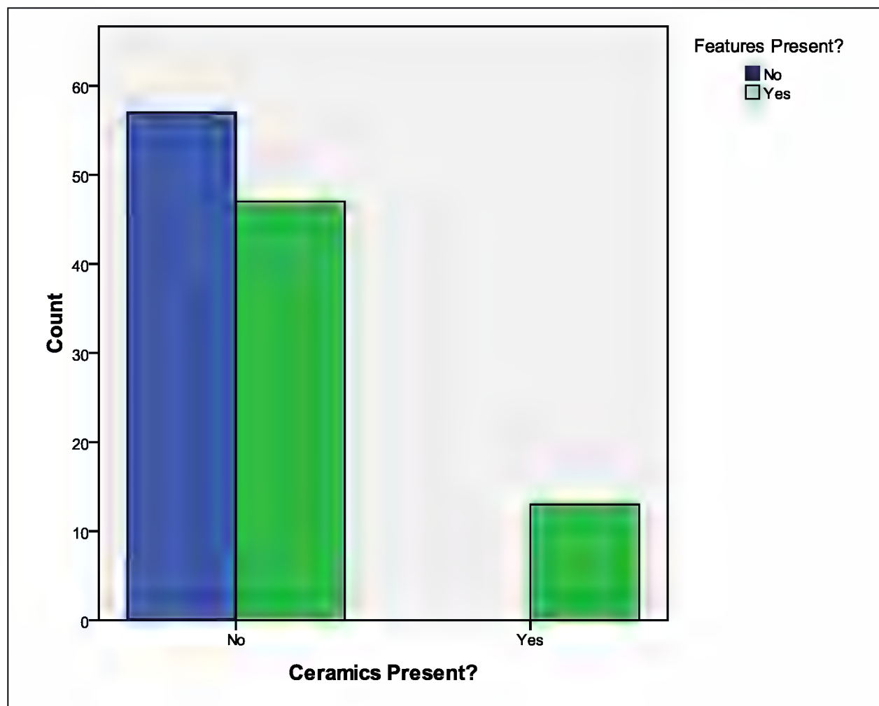
Figure 20. Number of analysis units with and without features, grouped according to whether ceramics are present.
