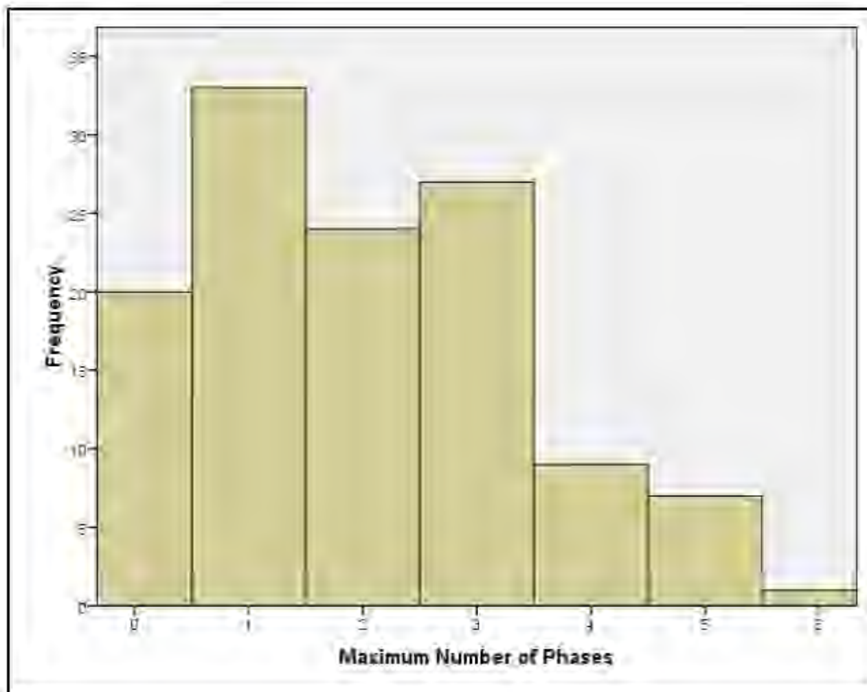
Figure 10. Distribution of maximum number of phases for analysis units in Table 19.
