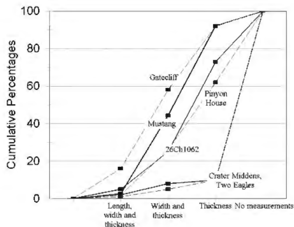
Figure 26. Cumulative curves showing the relationship between Mustang Shelter's overall biface completeness curve and those of other selected sites.
