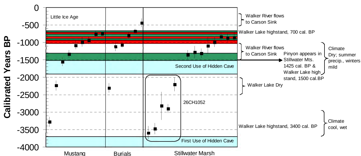
Figure 50. The distribution of dates, with two sigma ranges, from Mustang Shelter, Stillwater burials and marsh sites (calibrated using CALIB 5.0.2; present = AD 2000). Green = Stillwater highs; red = droughts. Other environmental events to the right.
