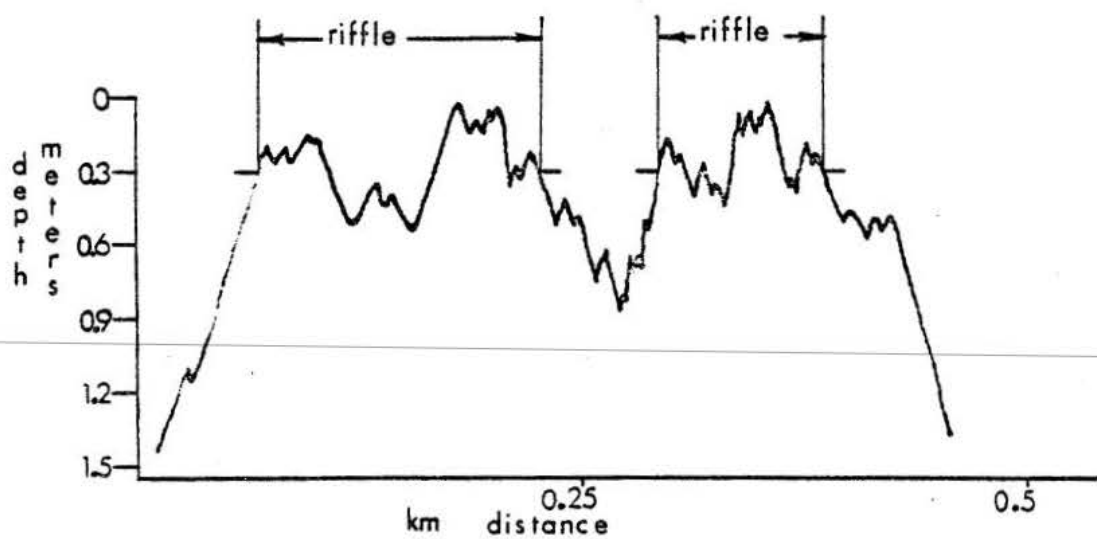
Figure 3. Illustration of fathometer record analysis/interpretation for riffles.
