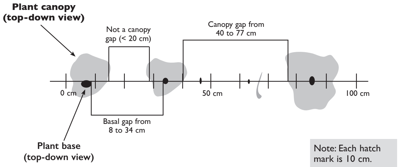
Figure 21. Example of canopy gap intercepts (above the line) and basal gap intercepts (below the line) for 1 m (100 cm) of a 25 m line. Canopy gaps: There is a gap between 40 and 77 cm because the plant canopies present do not cover more than 50% of any 3 cm segment. Basal gaps: There is a basal gap between 8 and 34 cm. Because the three small plant bases between 34 cm and 86 cm are all within 20 cm of an adjacent plant base, there are no canopy gaps even though there is a basal gap.
