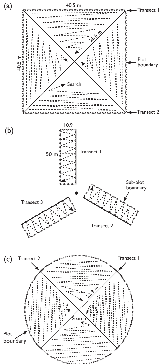
Figure 36. Three species inventory plot layout options to achieve an area of 1,641 m 2 : (a) a single square species inventory plot with a side of 40.5 m (132.9 ft), (b) three 10.9 (35.7 ft) x 50 m (164 ft) rectangular sub-plots, and (c) a 22.9 m (75 ft) radius, circular plot. Dashed lines represent the path walked by the observer.
