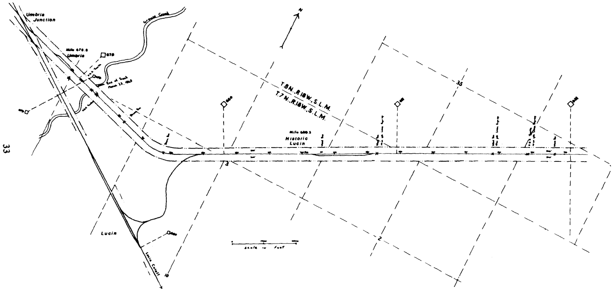
Figure 21: Umbria and Lucin (compiled from Southern Pacific Railroad plats, station plans, and profiles).
