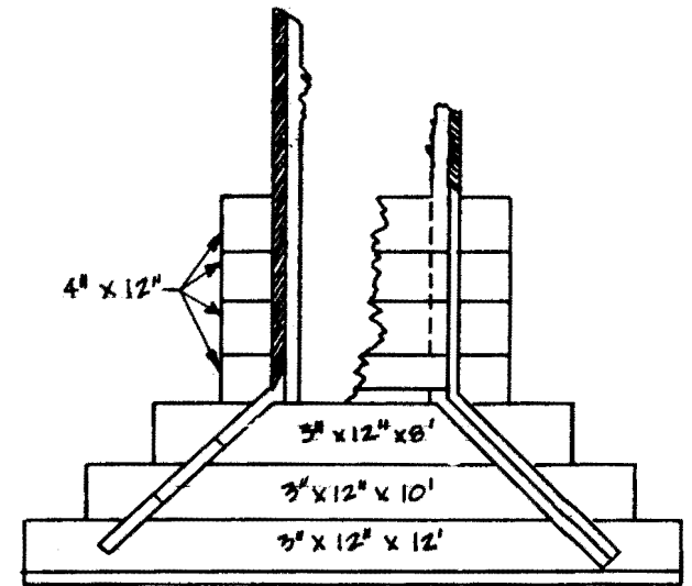
PLAN OF END
