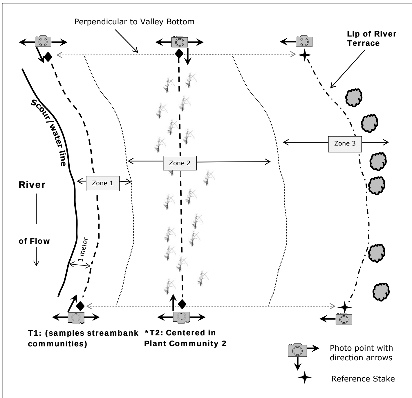
Figure 6. DMA Configuration (C Complex Types). Transects do not need to correspond to zones. Zones are displayed for reference only.
