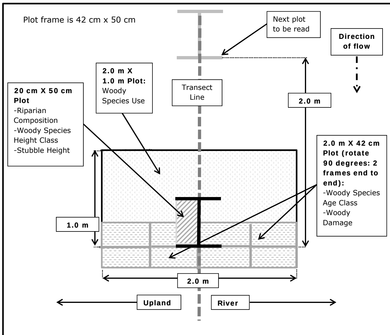
Figure 10. Plot layout
