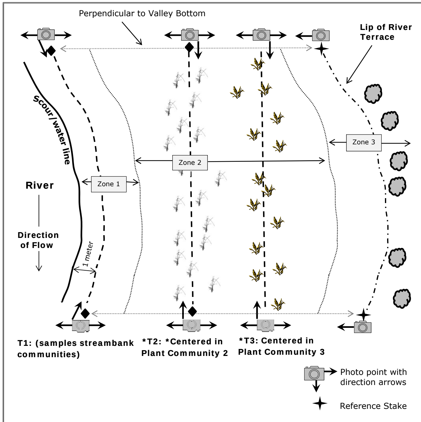
Figure 7. DMA Configuration (D Complex Types). Transects do not need to correspond to zones. Zones are displayed for reference only. Transects do not need to be precisely parallel to each other as shown. The exact orientation is established after top and bottom markers are located in the center of the plant community.
