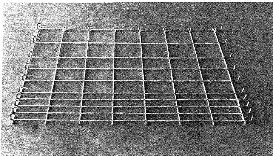
Picture 1 - Panel type 1 (32 inches x about 4 feet). One of these panels is needed for each cage. Note the hook design on both ends of this panel (corner hooks on the left and closing hooks on the right).
