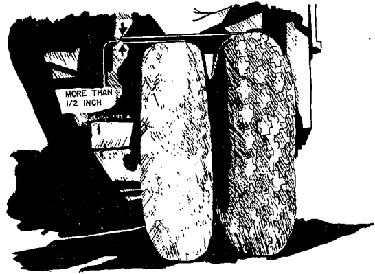
Difference in diameter for duals.
