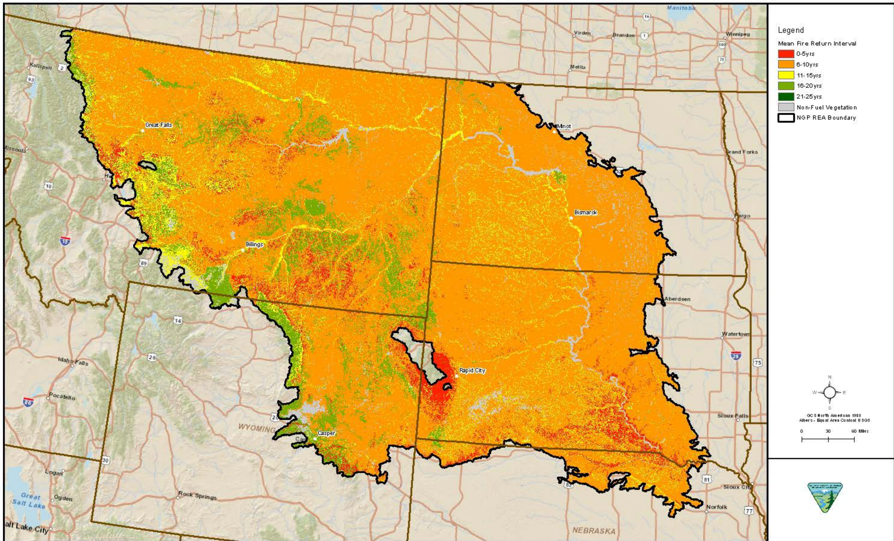
Figure C-2-9. Mean Fire Return Interval
