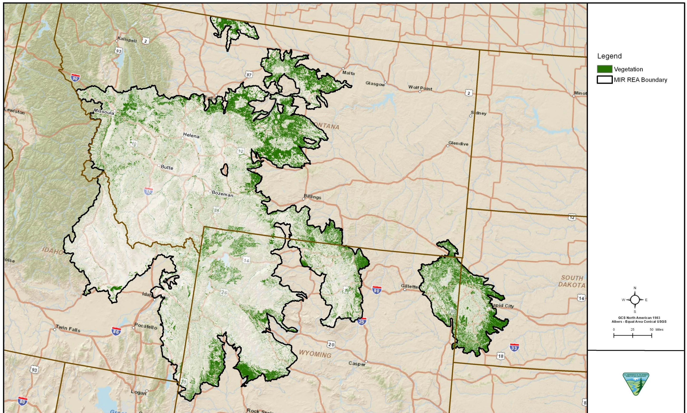
Figure C-3-33. Leafy Spurge ReGAP Level 2/Level 3 Classifications
